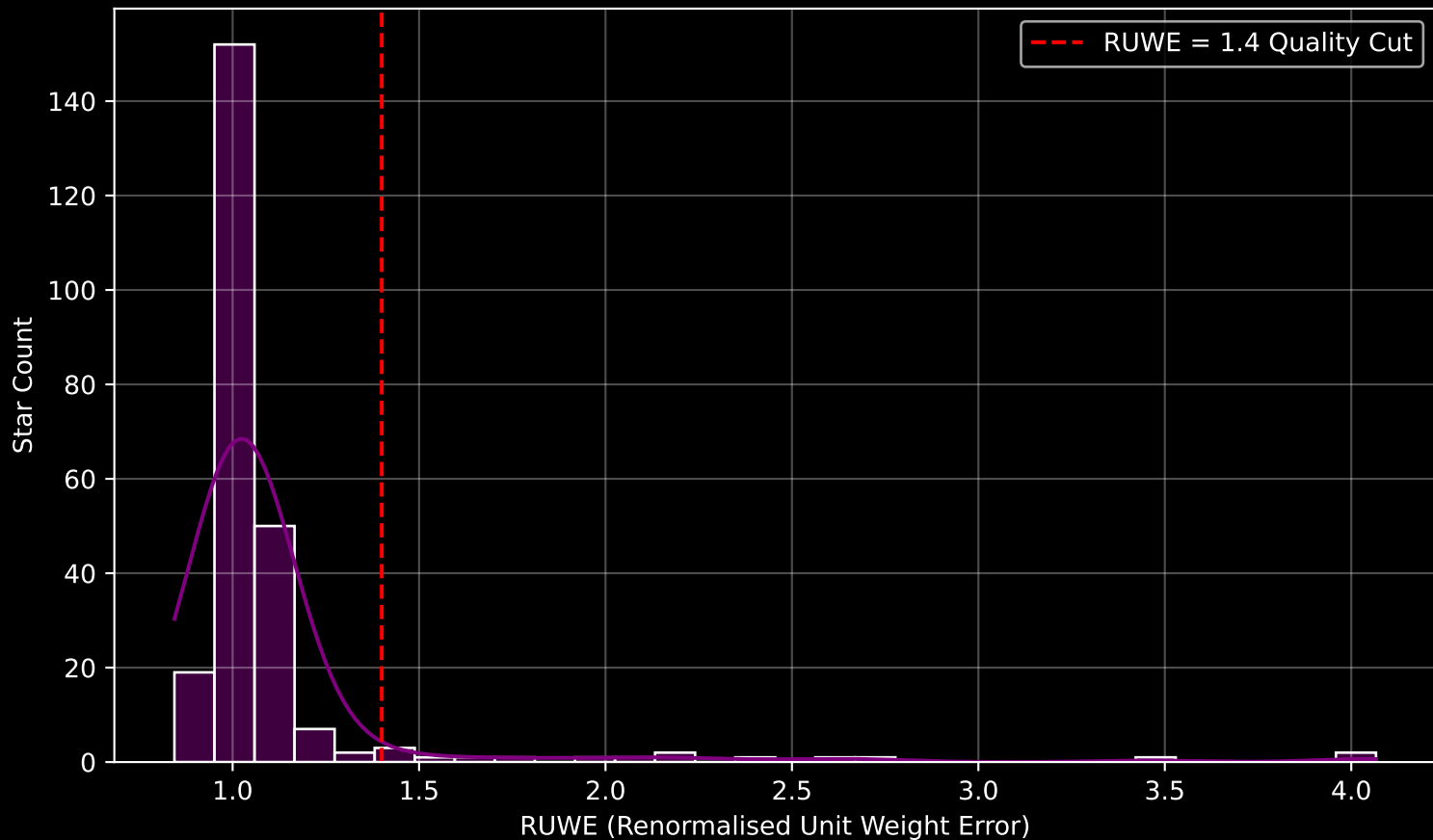
GAPOGEE DR17 Field [Berkeley_2_btx] RUWE Distribution (n= 246)
