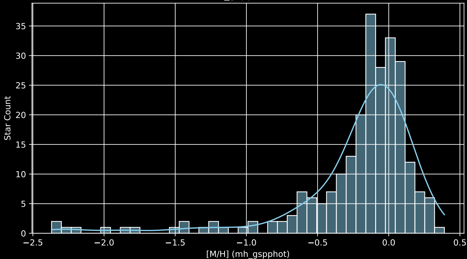
APOGEE DR17 Field: [Berkeley_2_btx [M/H] (mh_gspphot) (n= 245)
