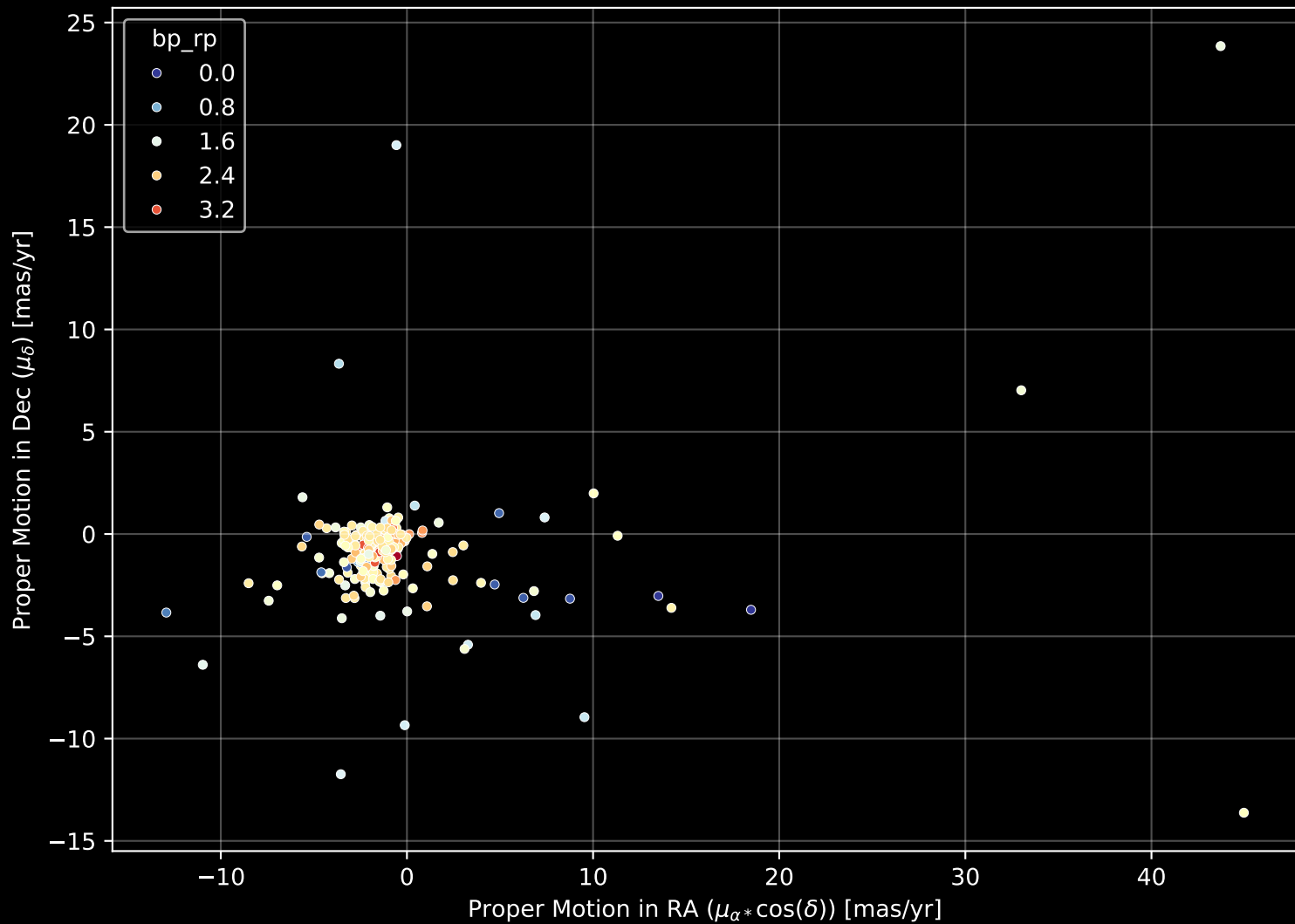
APOGEE DR17 Field: [Berkeley_2_btx] Proper Motion Diagram (n= 252)
