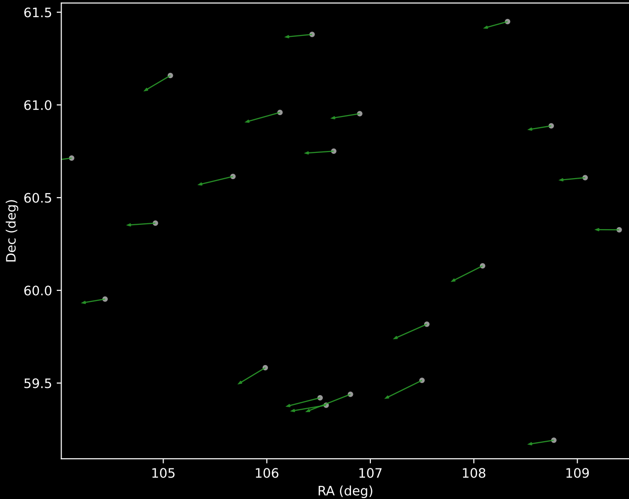
APOGEE DR17 Cluster 4 Proper Motion Vectors (n=21)
