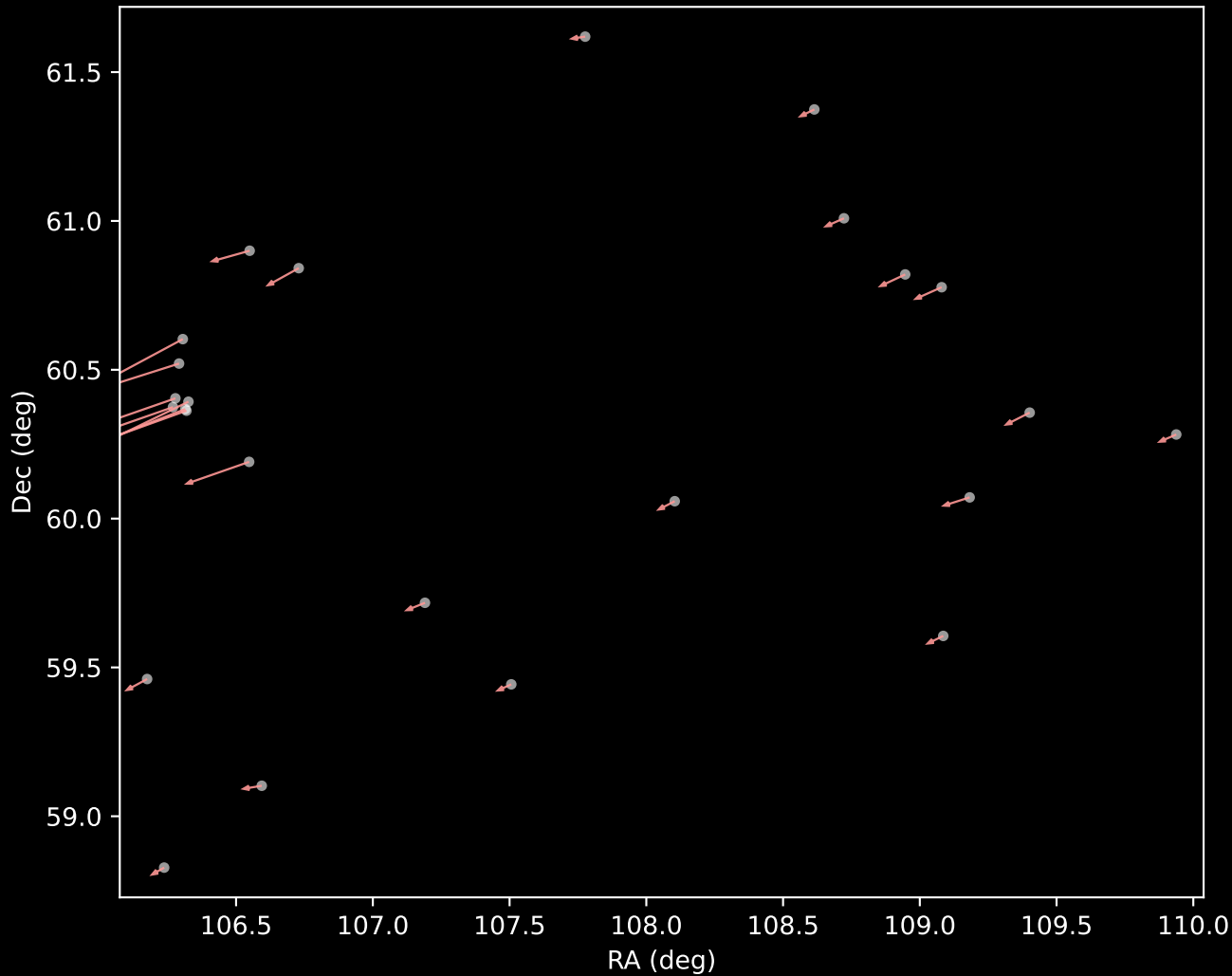
APOGEE DR17 Cluster 7 Proper Motion Vectors (n=25)
