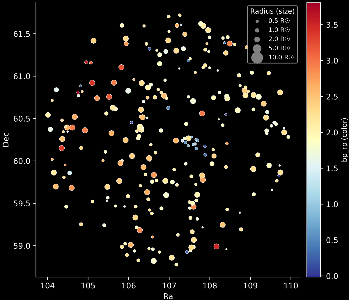
APOGEE DR17 Field: [Berkeley_2_btx] Stars: 252
