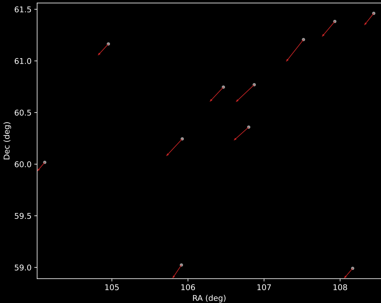
APOGEE DR17 Cluster 6 Proper Motion Vectors (n=11)
