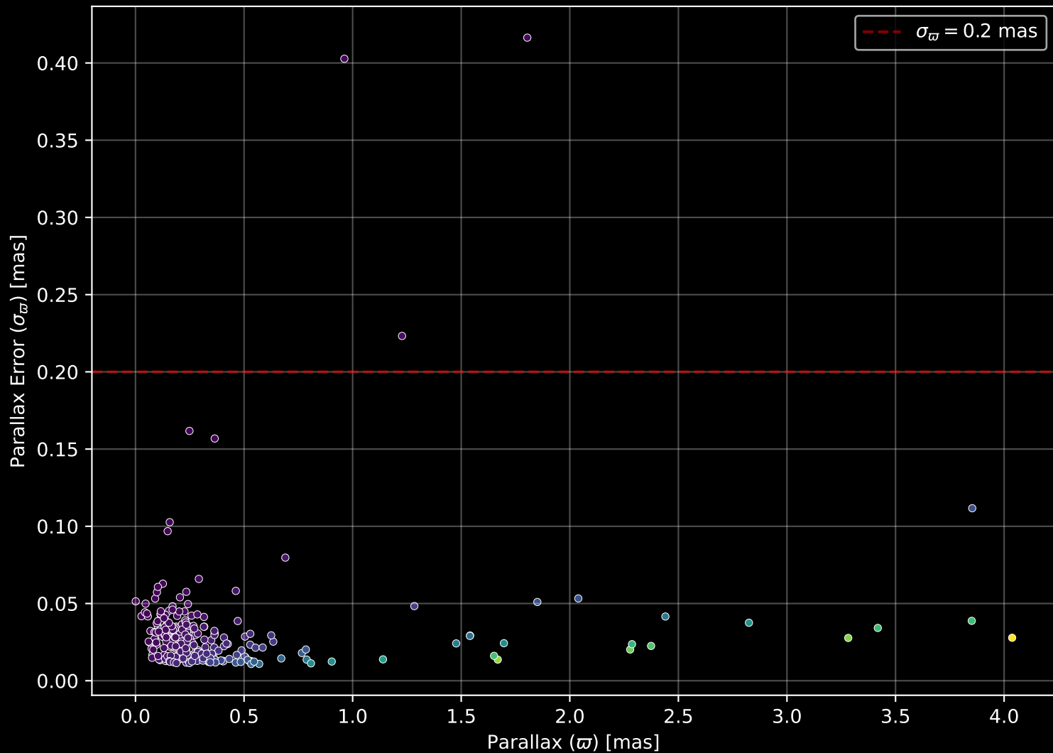
APOGEE DR17 Field: [Berkeley_2_btx] Parallax Quality (n= 252)
