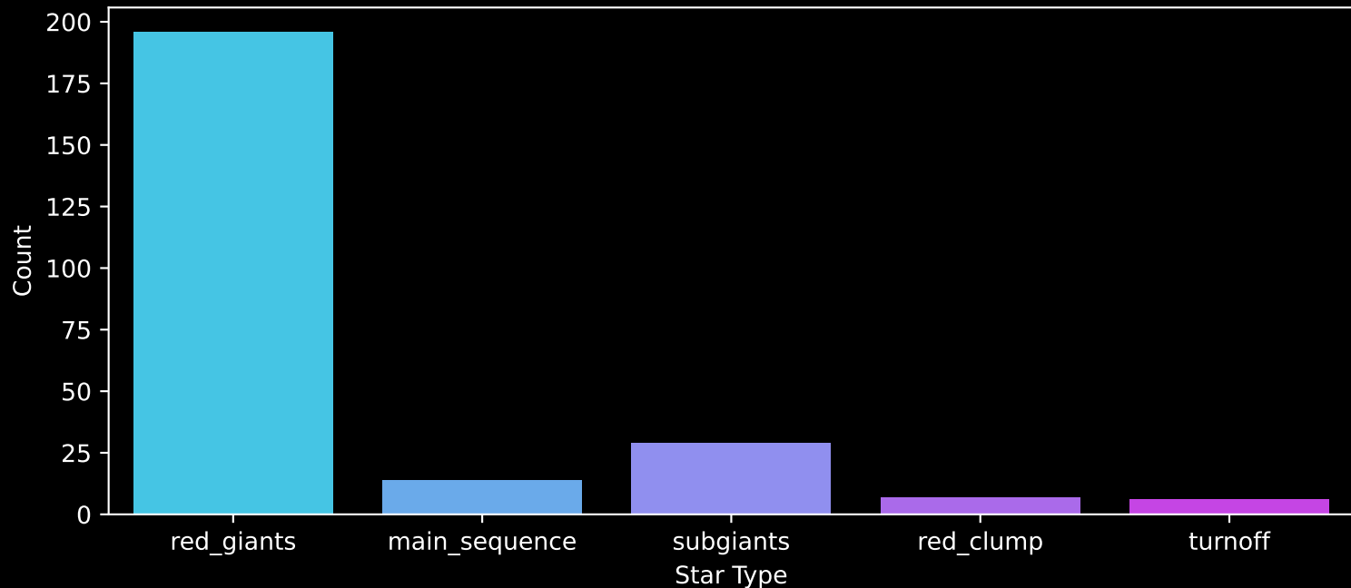
APOGEE DR17 Field: [Berkeley_2_btx] Count plot of Star Type
